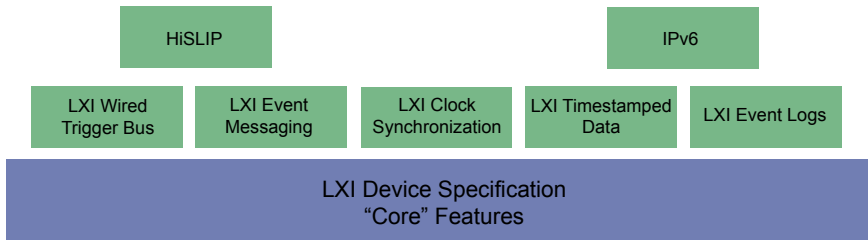
Fig. 1.1 - The LXI 1.4 Structure showing the Extended Functions
