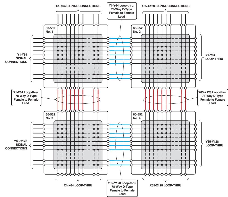
Fig. 11.7 - 100x100 Matrix using 4 x 60-552 LXI Units
